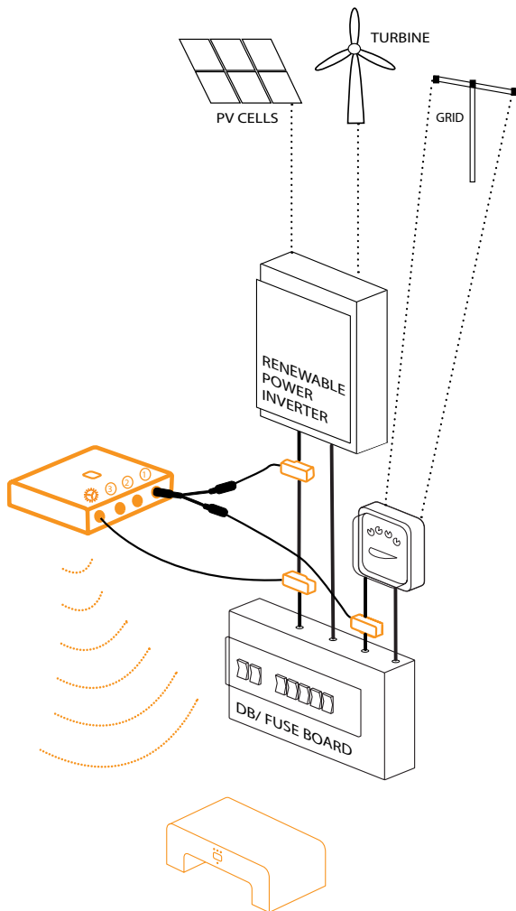
Wattson Solar Plus installation with Easifit
