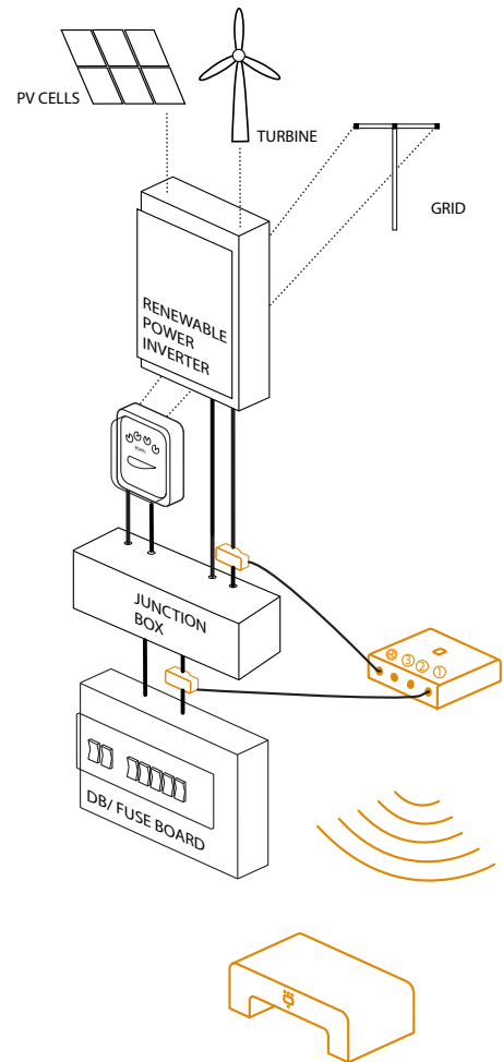
Wattson Solar Plus with Henley Block or junction box
